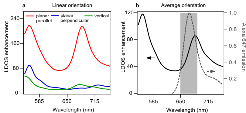
Figure 5. Numerical simulations of LDOS enhancement for a dipolar emitter located in the center of the DNH gap. In (a), three different dipole orientations are displayed, the case when the dipole is oriented parallel to the apex provides the highest LDOS enhancement. In (b), the orientation-averaged LDOS enhancement is plotted as function of the emission wavelength (solid line). The normalized Alexa Fluor 647 emission spectrum is shown in dashed gray line, and the 650–690 nm region used experimentally for fluorescence collection is indicated.
