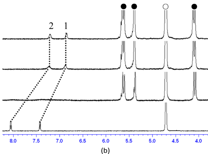
Fig. 2. (a) The ^1\text{H} NMR titration spectra of BZC in the presence of increasing amounts (0, 0.5, 1.2, 2.2, 3.1 equiv.) of CB[7] at \text{pD} = 2 ; (b) The ^1\text{H} NMR titration spectra of PABA in the presence of increasing amounts (0, 0.7, 1.5, 3.0 equiv.) of CB[7] at \text{pD} = 2 . The peaks labelled as (●) and (○) are CB[7] and HOD protons, respectively.
