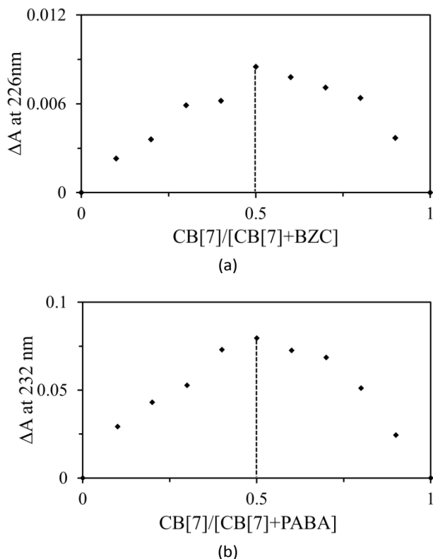
Fig. 4. (a) Job's plot based on a UV-visible continuous variation titration and monitored by the changes in the UV-visible absorbance at 226 nm with [CB[7]] + [BZC] = 0.05 mM in aqueous solution (pH = 2); (b) Job's plot based on a UV-visible continuous variation titration and monitored by the changes in the UV-visible absorbance at 232 nm with [CB[7]] + [PABA] = 0.2 mM in aqueous solution (pH = 2). The maximum exhibited at 0.5 indicates the formation of 1:1 complexes between the guest and the host.
