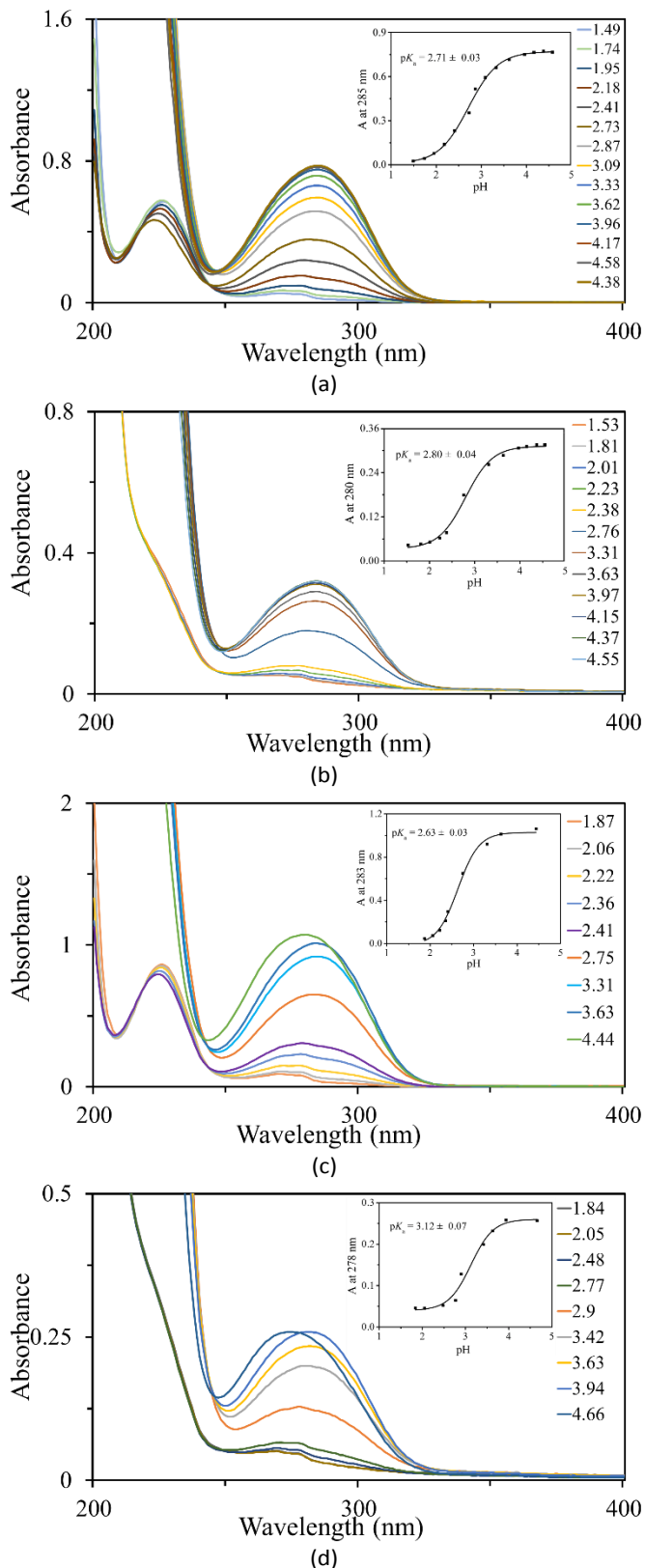
Fig. 6 Plots of pH-dependent UV-Visible titrations for determining pK_a values of BZC and PABA in the absence and presence of 20 equivalents of CB[7]; (a) BZC; (b) BZC with CB[7]; (c) PABA; (d) PABA with CB[7]. The concentration of each guest is \sim 0.1 mM.
