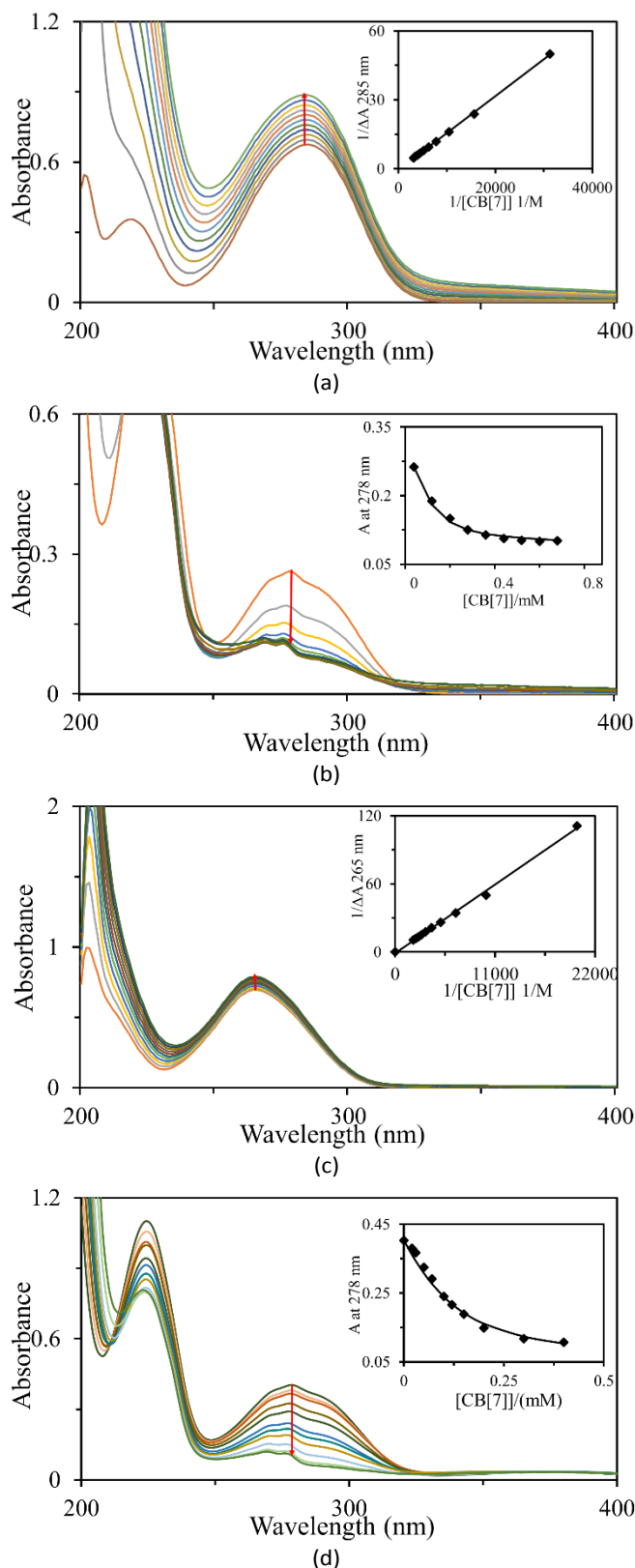
Fig. 5. UV-vis titration of BZC with increasing amounts of CB[7] in PBS buffer (pH = 7.4) (a); HCl solutions (pH = 2) (b); UV-vis titration of PABA with increasing amounts of CB[7] in PBS buffer (pH = 7.4) (c); HCl solution (pH = 2) (d). The insets in the four figures show the best fit between experimental points and a 1:1 binding model affording a binding constant K_a of \sim 300 \text{ M}^{-1} , 2.2 \pm 0.2 \times 10^4 \text{ M}^{-1} , 200 \text{ M}^{-1} and 1.5 \pm 0.2 \times 10^4 \text{ M}^{-1} respectively.
