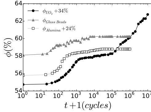
Figure 1: Examples of experimental results under horizontal vibrations at 100 Hz and 7g acceleration. The tank was 15 \times 15 mm 2 .
