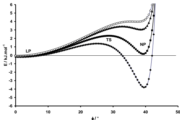
Figure 2. E = E_{dih} + E_{disp} as a function of the dihedral angle \phi for different V/\varepsilon ratios. The minimum at \phi=0 represents the open structure LP, the other minimum represents the NP structure. There is a barrier (Transition State) between the minima indicated as TS. Losange: V/\varepsilon=1.7 . Squares: V/\varepsilon=2.5 . Triangles: V/\varepsilon=4 . Circles: V/\varepsilon=5 .
