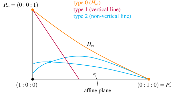
Fig. 1.1 Lines in \mathbb{P}(1, a_1, a_2) .
