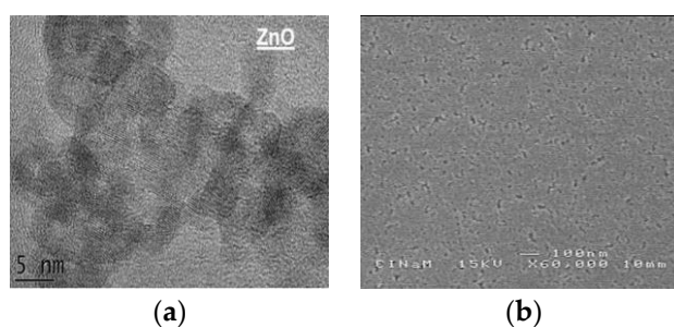
Figure 1. (a) TEM image of ZnO nanospheres at 30 mg/mL with 0.2% ethanolamine and (b) SEM image of a spin-coated ZnO thin film as S2 and post-annealed at 80 °C.
