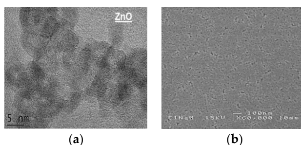
Figure 1. (a) TEM image of ZnO nanospheres at 30 mg/mL with 0.2% ethanolamine and (b) SEM image of a spin-coated ZnO thin film as S2 and post-annealed at 80 °C.
