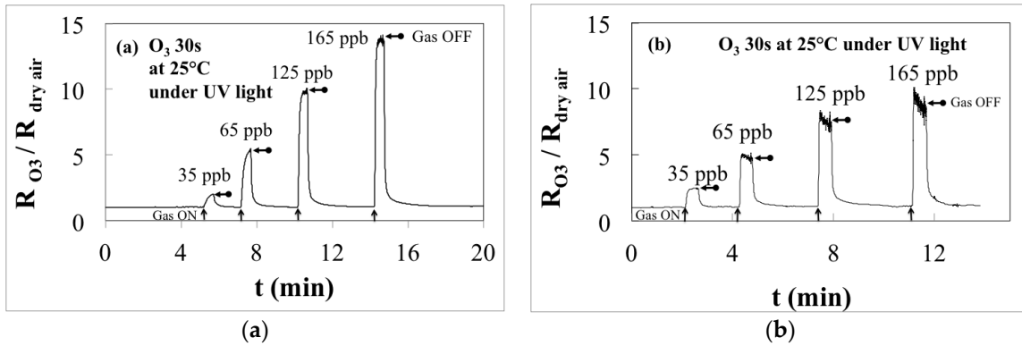
Figure 2. Normalized responses at 25 °C for O 3 sensors based on ZnO at 30 mg/mL (post-annealed at 80 °C) under UV light (a) without EA (S1) and (b) with EA (S2).
