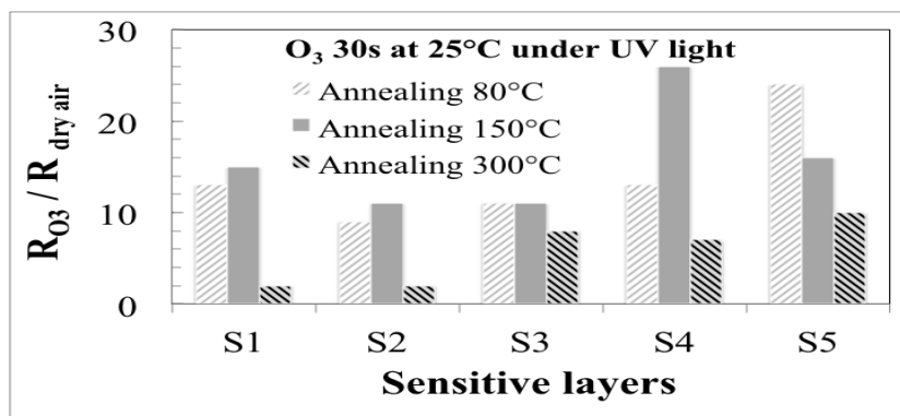
Figure 4. Sensor responses for 165 ppm of O 3 at 25 °C under UV light for three post-annealing temperatures.
