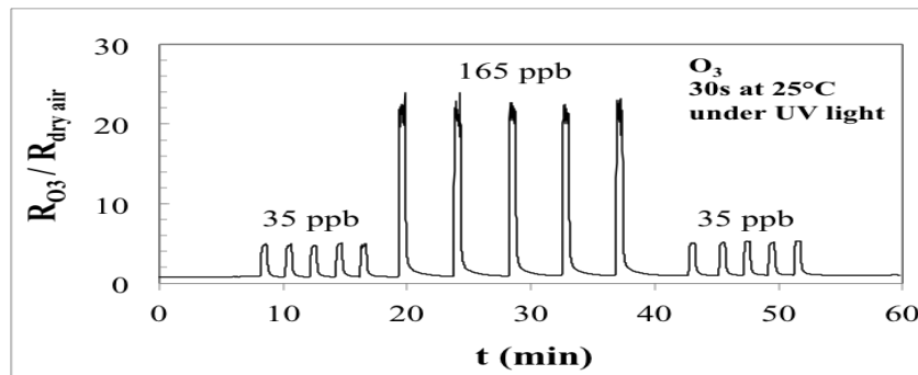
Figure 3. Repeatability of a 200 nm thick sensor with a sensitive layer based on ZnO at 30 mg/mL with EA (S5) and post-annealed at 80 °C, working at 25 °C under continuous UV illumination for 35 ppb and 165 ppb of O 3 .
