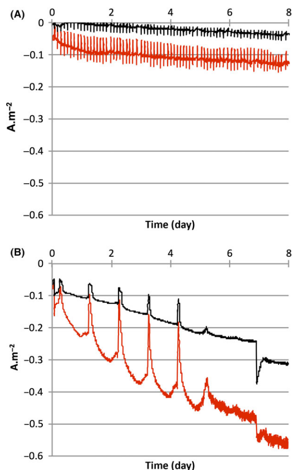
Fig. 2. Chronoamperograms of 3 cm 2 pre-colonized carbon felt bi-cathodes. Sulfur (A) or ferrous iron (B) was used as the prior energy source, either with C14-AHLs (red lines) or without C14-AHLs (black lines). CA was performed on MPG-2 potentiostat (Biologic) at E = -0.2 V versus Ag/AgCl KCl saturated reference and T = 30^{\circ}\text{C} .
