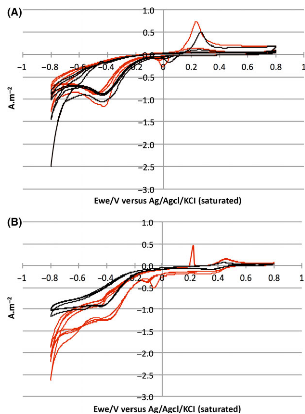
Fig. 3. Cyclic voltammetry plots for five consecutive cycles of bio-cathodes. Electrodes were formed by using either sulfur (A) or ferrous iron (B) as the prior energy source, either with C14-AHLs (red lines) or without C14-AHLs (black lines). CV curves were obtained at a scan rate of 5 \text{ mV s}^{-1} .
