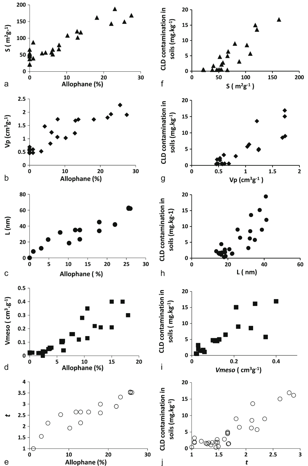
Fig. 3 Increase of the specific surface area S (a), the total pore volume V_p (b), the size of the fractal aggregate L (c), the mesopore volume V_{meso} (d), and the tortuosity t (e), with allophane content. And, increase of soil contamination with specific surface area S (f), total pore volume V_p (g), the size of the fractal allophane aggregates L (h), the mesopore volume V_{meso} (i), and the tortuosity t (j)
