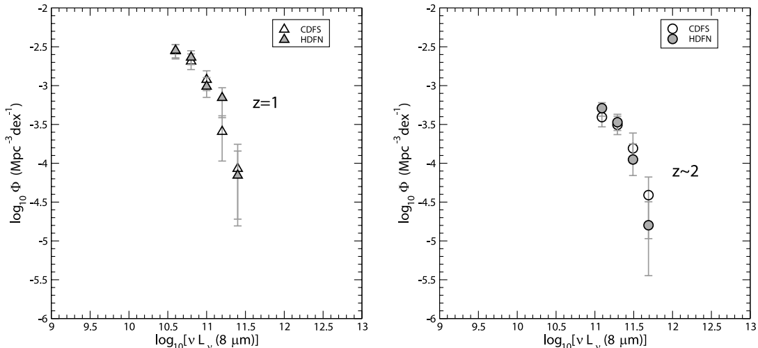
FIG. 9.—Rest-frame 8 \mu\text{m} LF for star-forming galaxies in the GOODS/CDF-S and HDF-N separated, as computed with the 1/V_{\text{max}} method. Left: z = 1 ; right: z \sim 2 .
