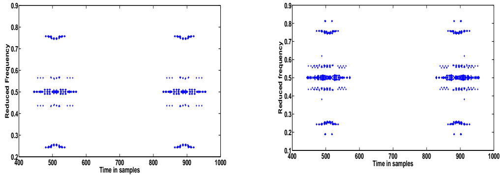
Figure 5. Delay-Doppler points selected with the detector C_{\text{Ins}} . left : SNR=100 dB. right : SNR=10 dB
