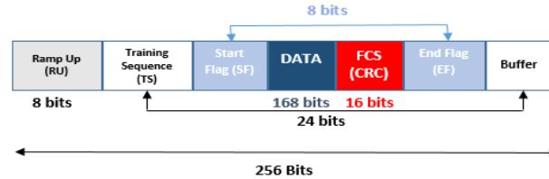
Figure 2. AIS Frame
