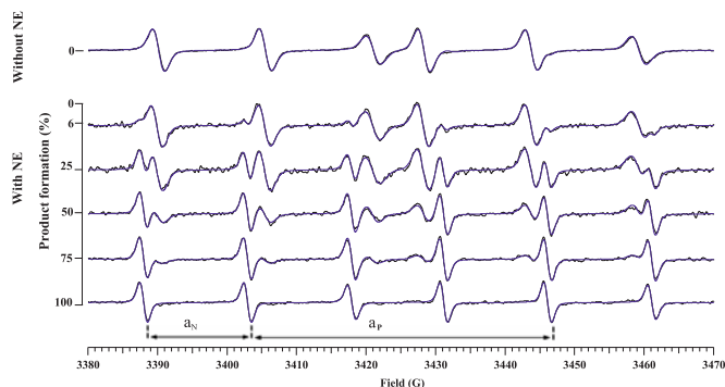
Fig. 1. EPR spectroscopy of the line-shifting nitroxide: hydrolysis of 40 \mu M substrate R-3 by 0.8 nM protease NE yielding the product R-1 . Five EPR spectra are represented corresponding to five reaction steps: 6%, 25%, 50%, 75% and 100% of product formation. Only 6% of product was formed after the first EPR acquisition. Spectrum without NE corresponds to substrate R-3 (0% of product) whereas spectrum with NE at 100% illustrates the product R-1 . Spectra (dark lines) are fitted by a linear combination of substrate and product (blue lines). Hyperfine coupling of the unpaired electron with the phosphorus atom 31 P (spin 1/2) and with the nitrogen atom 14 N (spin 1) provide 6 EPR lines. Parameters a_P and a_N are phosphorus and nitrogen coupling constants deduced from EPR product or substrate spectra. (For interpretation of the references to color in this figure legend, the reader is referred to the web version of this article.)
