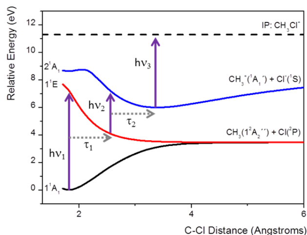
Figure 7. Scheme of a sequence of three time-resolved ultra-short laser pulses for detection of the \text{H}_2\text{CH}^+\cdots\text{Cl}^- complex. Only the relevant states are shown.
