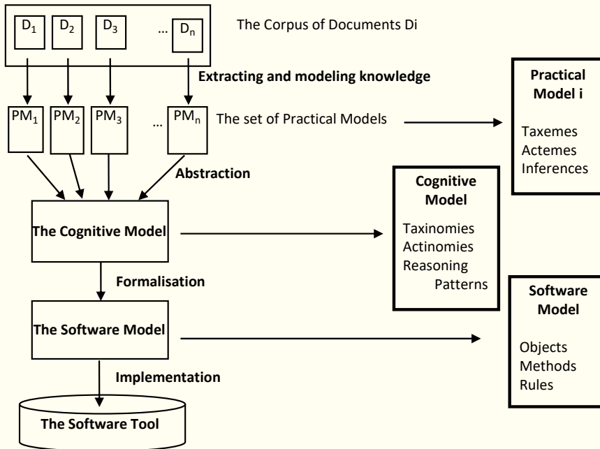
Figure 4: The KOD design process
