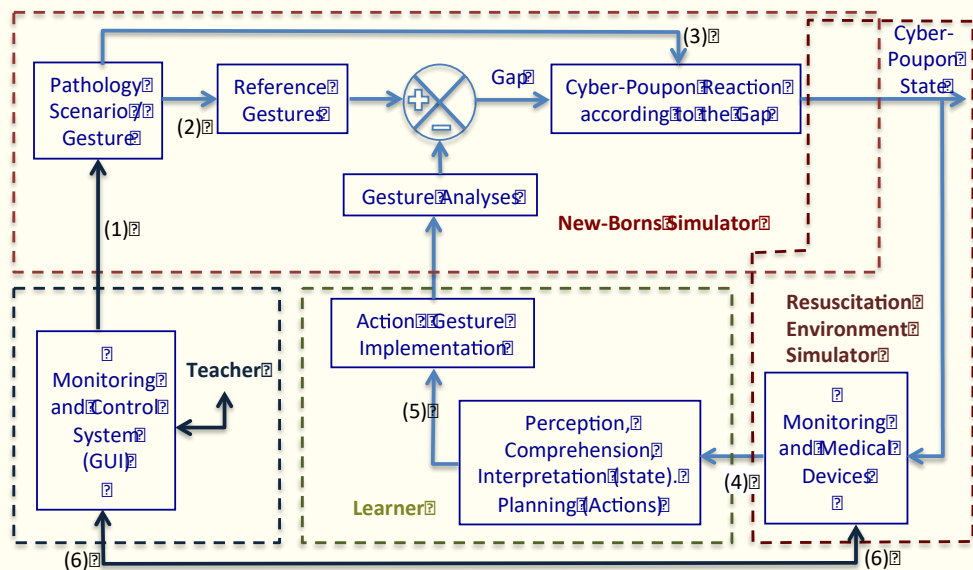
Figure 2: Functional diagram of the new-borns simulation system. Relationships labelled with a number between brackets (n) are detailed in the above paragraph.
