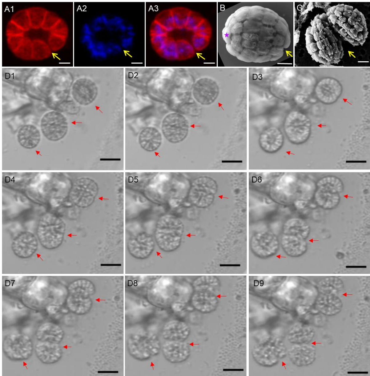
Fig. 3 UV triggered division of magnetoglobules. (A) images of fluorescence microscopy of a Mediterranean ellipsoidal magnetoglobule by FM-4-64 staining (red color, A1) to visualize membranes and DAPI staining (A2) to visualize chromosomes (blue spots); A3 is a superposition of A1 and A2. (B) is the SEM image of a Mediterranean ellipsoidal magnetoglobule. Yellow arrows indicate the initiation sites of the division, and the purple star shows the cells at the end opposite to the division initiation site. (C) is a SEM image of an ellipsoidal magnetoglobule, collected from the China Sea, at the end stage of the unidirectional division. (D) is the process of UV-triggered division of 3 Mediterranean ellipsoidal magnetoglobules. The duration from D1 to D9 is 315 sec. Scale bars: 2 \mu\text{m} in A, B, and C, and 10 \mu\text{m} in D.
