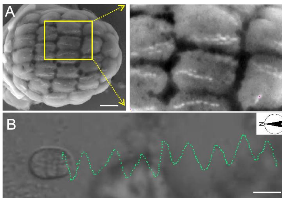
Fig. 1 Swimming behaviour of ellipsoidal Mediterranean magnetoglobules. (A) SEM shows magnetosomes (white particles) that organize in multiple chains in the magnetoglobules. (B) Magnetoglobules exhibit a north-seeking helical swimming trajectory. The bars are 1 \mu\text{m} and 10 \mu\text{m} in A and B, respectively.
