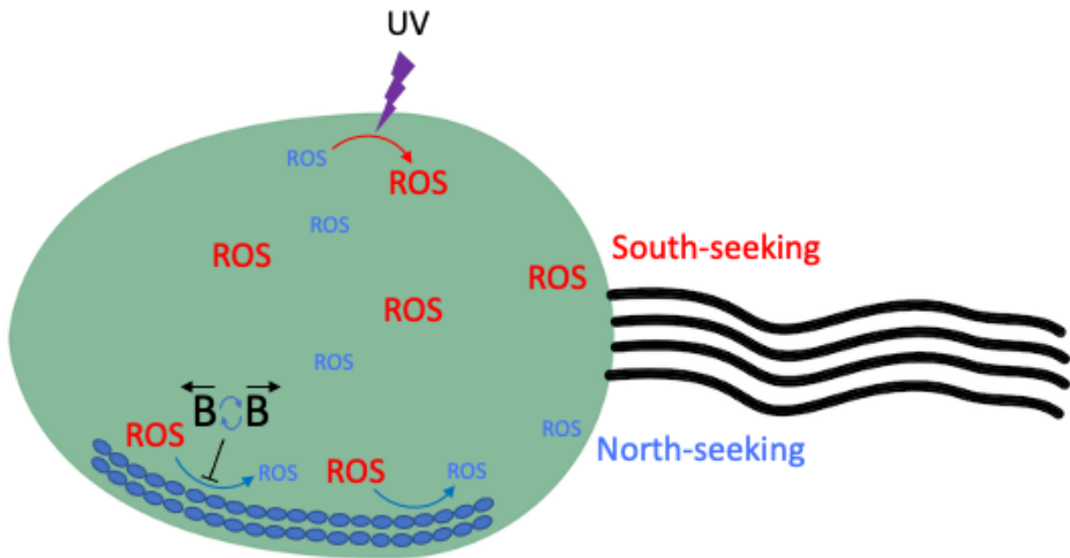
Fig. 4 Intracellular level of ROS might affect the swimming direction of magnetoglobules. The equilibrium of ROS level depends on magnetosome-catalyzed decrease of ROS (from big red ROS to small blue ROS, (Li, et al., 2017) and UV-generated ROS (from small blue ROS to big red ROS). At low level magnetoglobules swim northward, and at a level higher than the threshold magnetoglobules reverse the swimming direction to southward. Magnetic torque might decrease magnetosome capacity of reducing ROS, which results in sudden reversal of magnetoglobule swimming direction.
