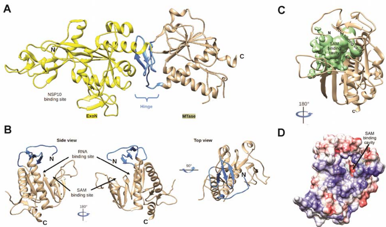
Figure 1. Global architecture of coronavirus nsp14 (PDB 5NFY). (A) Architecture of SARS-CoV nsp14 showing the N-terminal ExoN domain (Yellow), inter-domain hinge (blue), C-terminal N7-MTase domain (brown). (B) Side and top view of the hinge region and N7-MTase domain. The three strands of the hinge (blue) protrude from the N7-MTase domain (brown). (C) Analysis of the volume of the N7-MTase active site, with the cavity highlighted in green. (D) Electrostatic surface representation of the CoV nsp14 hinge region and N7-MTase domain. Surface electrostatic potential calculated by Adaptive Poisson-Boltzmann Solver, from - 10 (red) to + 10 (blue) kT/e.
