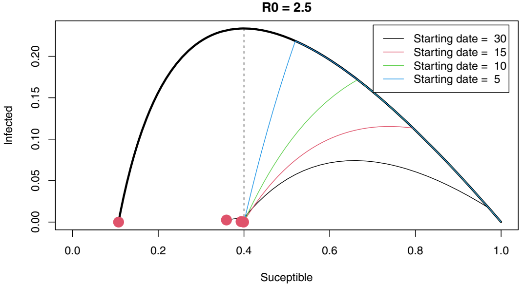
FIGURE 2 Phase diagram of optimal lockdown policies with different starting dates. Notes: Herd immunity corresponds to the dashed vertical line. The black thick line corresponds to the original trajectory of the epidemic. Starting date is the distance the peak
