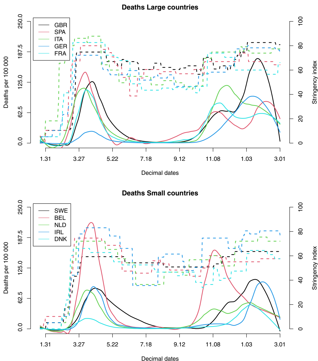
FIGURE 5 Deaths and policy reactions for large and small countries. Notes: The solid lines represent the smoothed normalized number of daily new deaths, using a loess regression. The dashed lines represent the severity index of governments' responses. Decimal dates correspond to month.day, while consecutive years 2020 and 2021 are not indicated. Source: University of Oxford, Blavatnik School of Government and authors' calculations. BEL, Belgium; DNK, Denmark; FRA, France; GBR, United Kingdom; GER, Germany; IRL, Ireland; ITA, Italy; NLD, the Netherlands; SPA, Spain; SWE, Sweden
