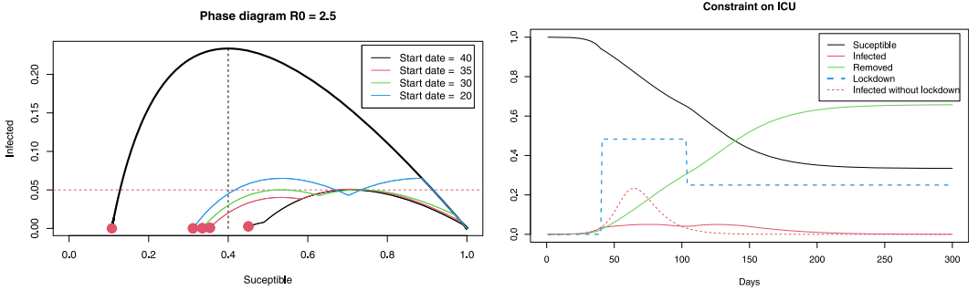
FIGURE 4 Waiting for a vaccine with a very long confinement. ICU, intensive care unit
