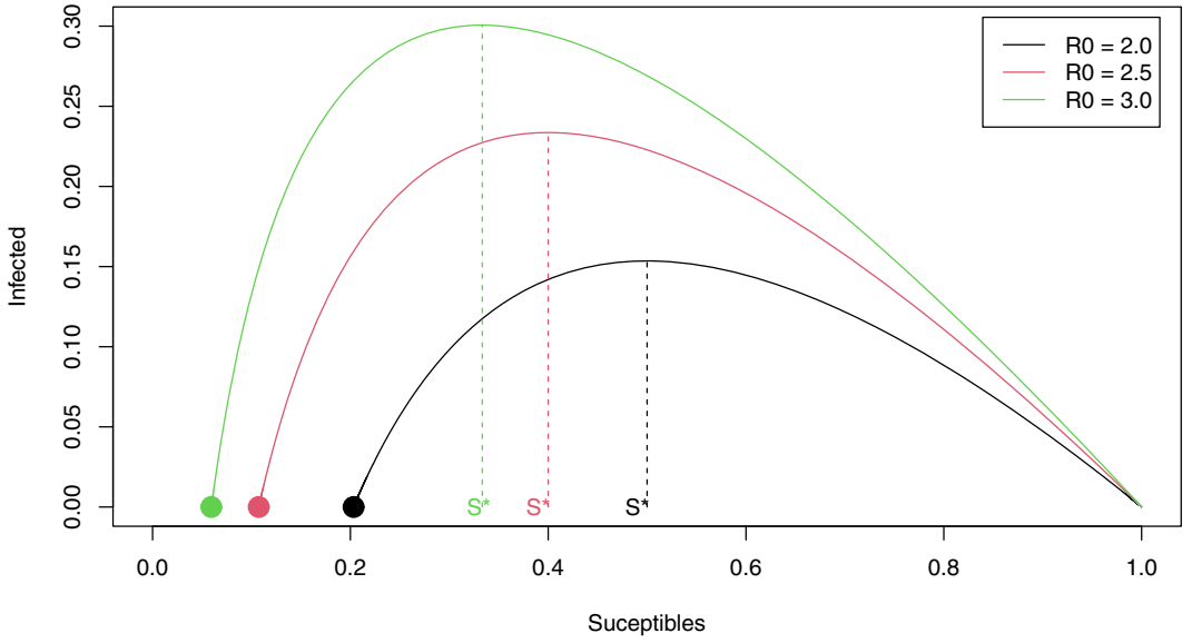
FIGURE 1 Overshooting after natural herd immunity. Notes: The vertical dashed lines represent both the peak of the epidemic and the level of herd immunity S^* . The dots indicate the end of the epidemic and the remaining proportion of susceptible S_\infty . Overshooting corresponds to the distance between S_\infty and S^* . Euler's method was used to solve the system of differential equations with a discretization step \Delta t = 0.01
