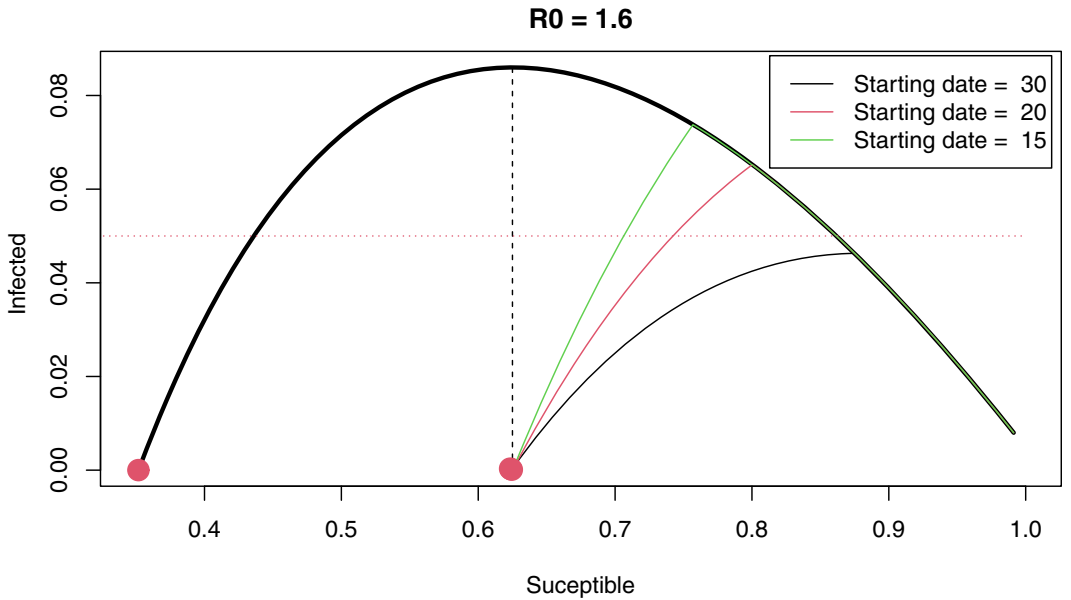
FIGURE 3 Optimal lockdown when \mathcal{R}_0 is low. Notes: Herd immunity corresponds to the dashed vertical line. The black thick line corresponds to the original trajectory of the epidemic. The red horizontal point line indicates the ICU capacity limit. Starting date is the distance to the peak. ICU, intensive care unit
