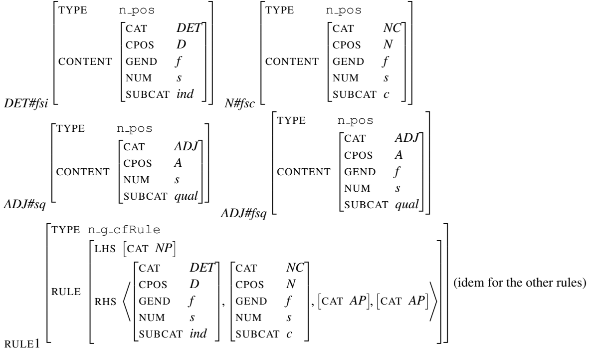
Figure 3: Alpha model: the syntactic relationships from the CFG in Fig. 2
