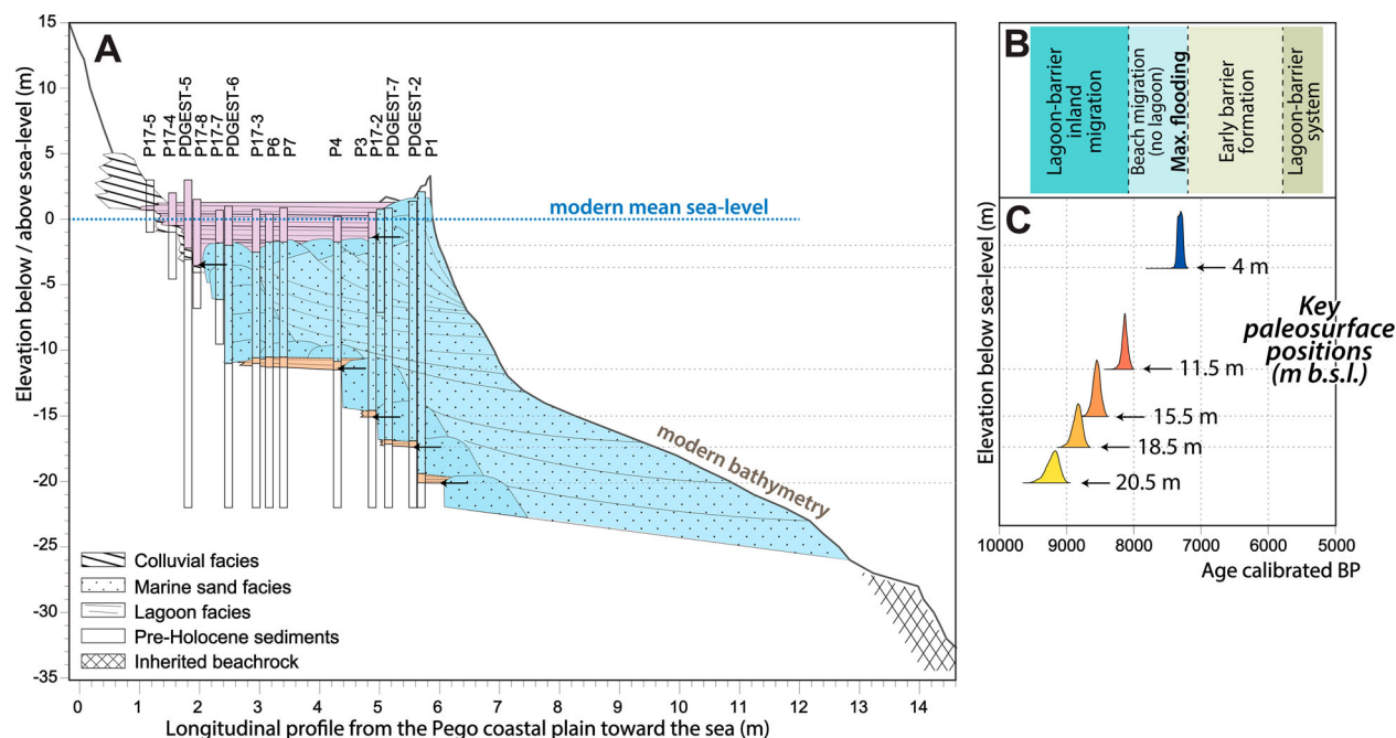
Figure 2. Main lithostratigraphic and geochronological results obtained for the Pego-Oliva coastal plain (Brisset et al., 2018). (A) Interpretative sketch of the sediment infilling signaling the presence of lagoon facies buried below the modern sea level at five key dates of the morphogenetic evolution. (B) Synthetic paleoenvironmental evolution during the Early to Mid-Holocene. (C) Age probability density function obtained for the five key dates of the morphogenetic evolution.
